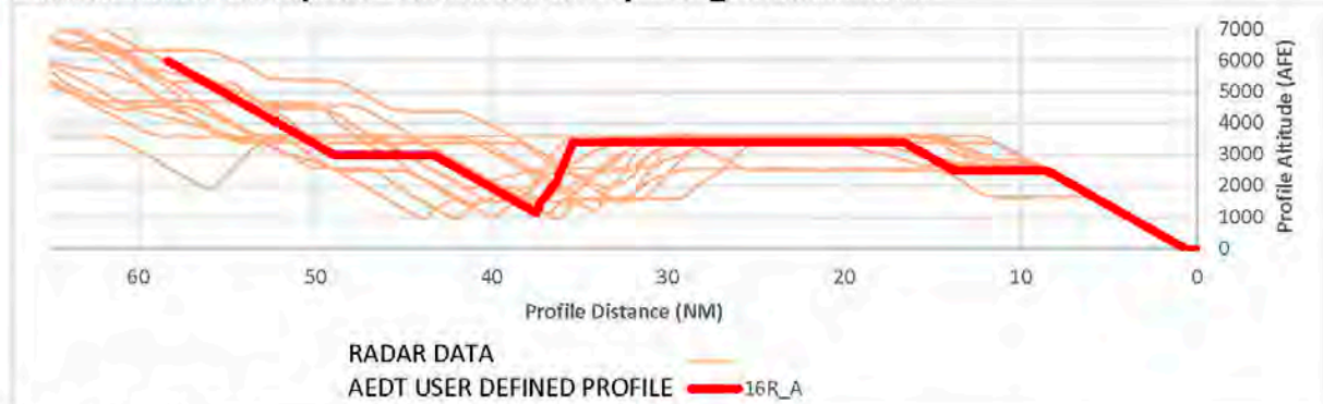
Exhibit 3: 737800 Runway 16R – Turn Before Runway – 16R_A Altitude Profile
