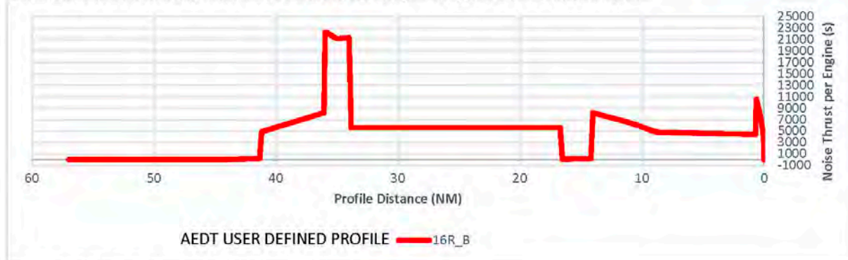
Exhibit 8: 737800 Runway 16R – Turn Before Runway – 16R_B Thrust Values Profile
