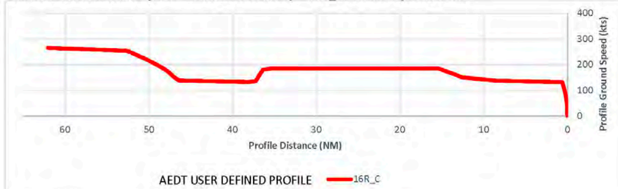
Exhibit 10: 737800 Runway 16R – Turn Over Runway – 16R_C Ground Speed Profile
