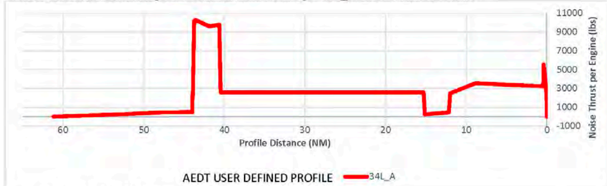
Exhibit 44: EMB 175 Runway 34L – Turn Before Runway – 34L_A Thrust Values Profile
