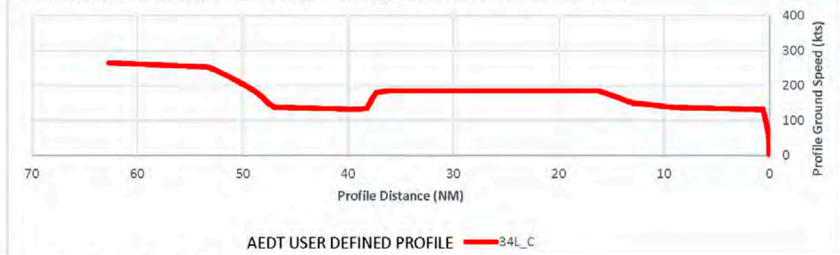
Exhibit 40: 737800 Runway 34L – Turn Over Runway – 34L_C Ground Speed Profile
