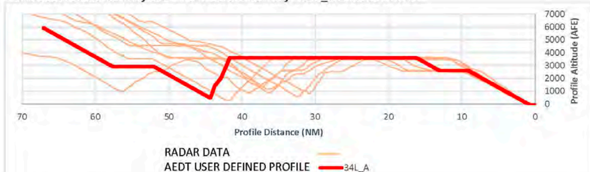
Exhibit 33: 737800 Runway 34L – Turn Before Runway – 34L_A Altitude Profile
